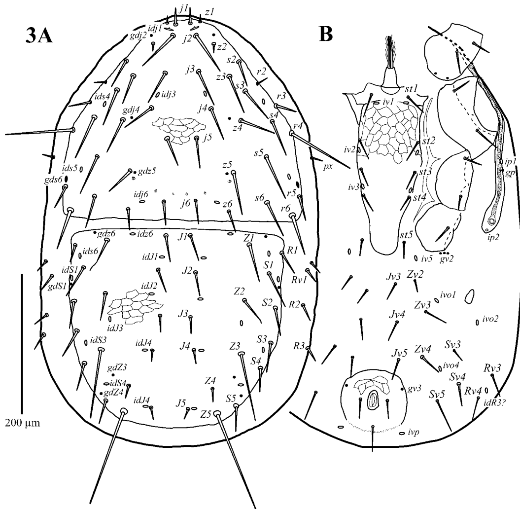
FIGURE 3. Euryparasitus occidentalis n. sp., deutonymph. A: dorsal view; B: ventral view.
