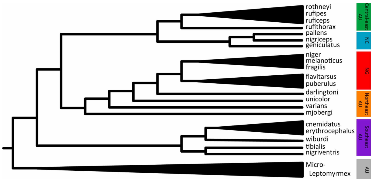
FIGURE 43. Simplified cladogram depicting relationships within the genus Leptomyrmex . Triangles represent species complexes not fully resolved by molecular phylogenetic analyses; AU = Australia, NC = New Caledonia, NG = New Guinea (modified from Lucky, in press).
