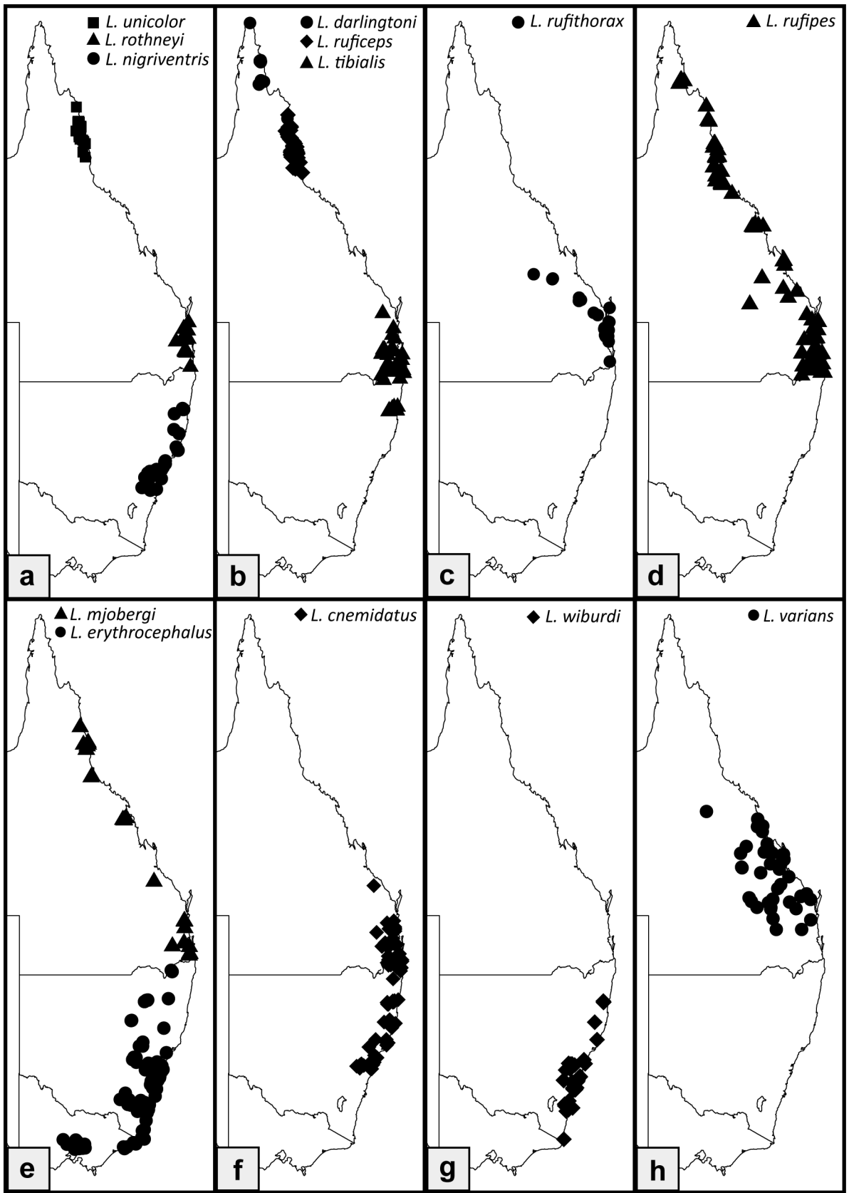
FIGURE 44. Geographic distribution of Australian macro- Leptomyrmex .
