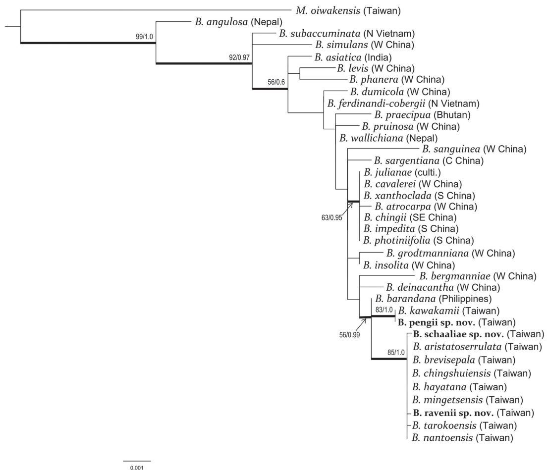
FIGURE 5. The best ML tree from the analysis of three concatenated chloroplast markers. Numbers adjacent to the nodes are ML bootstrap supports (BS) and BI posterior clade probabilities (PP). The well supported clades are denoted by thick line (BS > 50 and PP > 0.6).
