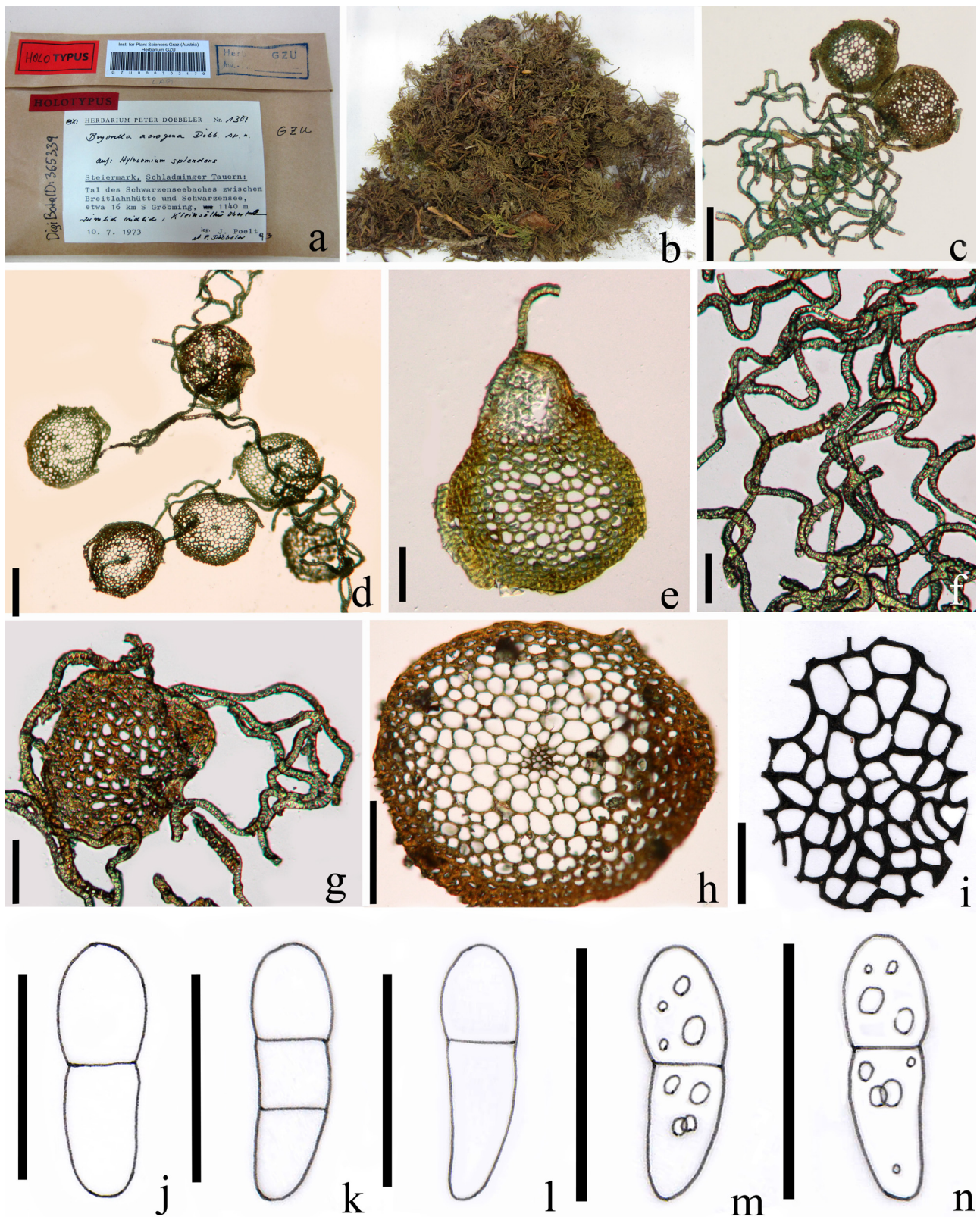
FIGURE 5. Bryorella acrogena (GZU000302179, holotype) a, b. Herbarium material. c, d, g. Ascomata with hypheae. e, h. Ascomata. f. Hyphae. i. Peridium. j–n. Ascospores. Redrawing of peridium and ascospore based on the original (Döbbeler & Melnik 1998) Scale bars: c–d = 200 μm, e, g–h = 100 μm, f = 50 μm, i–n = 15 μm.
